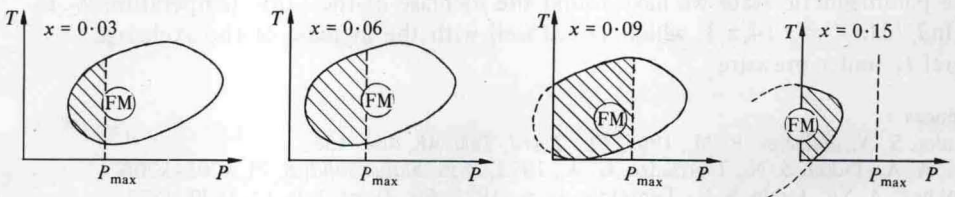
Figure 3. Shift of the ferromagnetic phase stability region (FM) in Mn_{1-x}Fe_xAs system with increasing value of x . The dashed area is the ferromagnetic phase stability region which was observed experimentally.
